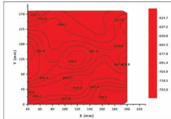
Fig 4. Half-Cell Potential at Steel Surface of Black Bars with Visible Corrosion at Bent Portion. (Potential is in mV)
