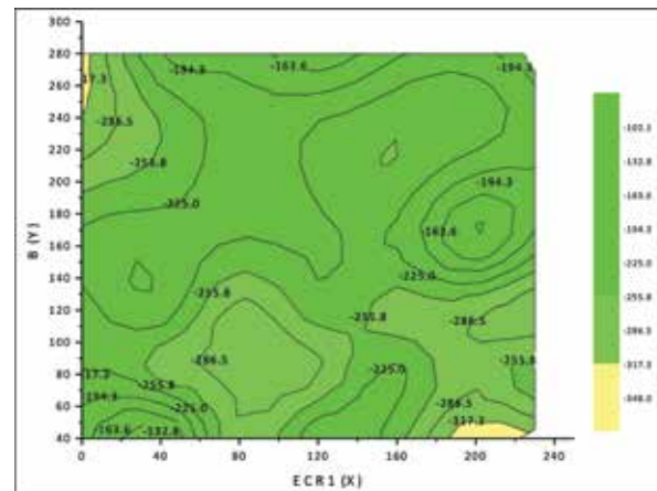
Fig 5. Half-Cell Potential of a Concrete Block with an Epoxy Coated Steel Bars without any Corrosion (Potential is in mV)
